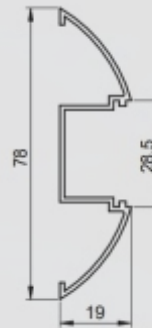
BUMPER Profile TEC 267
