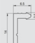
Fixing Profile TEC 180
